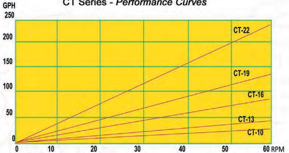
CT Series - Performance Curves
